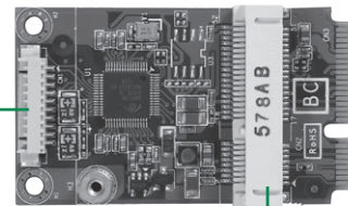
Full-size PCI Express Mini Card (PCIe only)
